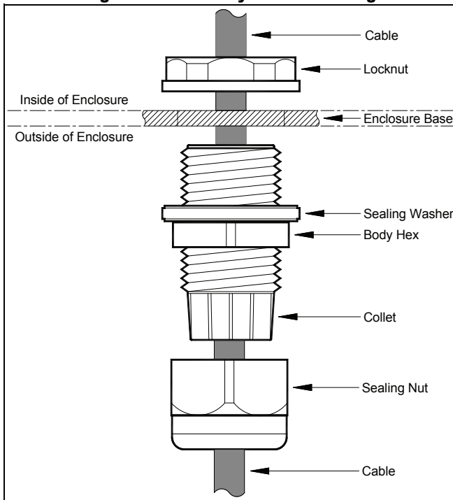
Figure 1 – Assembly Order of Fitting
