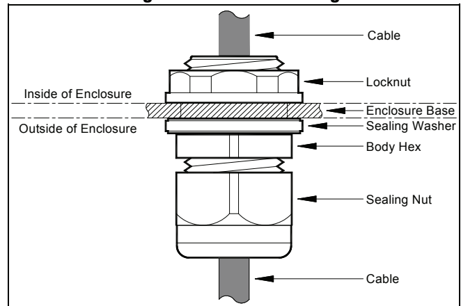
Figure 2 – Installed Fitting
